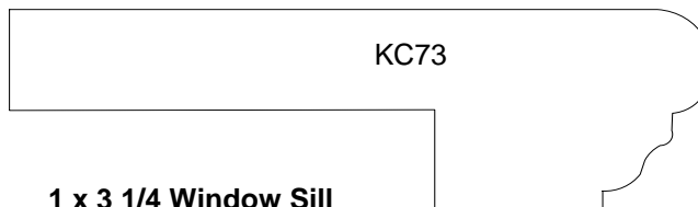
KC73 1 x 3 1/4 Window Sill
